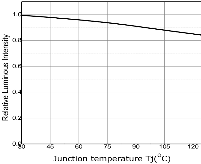
Fig 6. Relative Light Output vs. Junction Temperature, I_F=100\text{mA}
