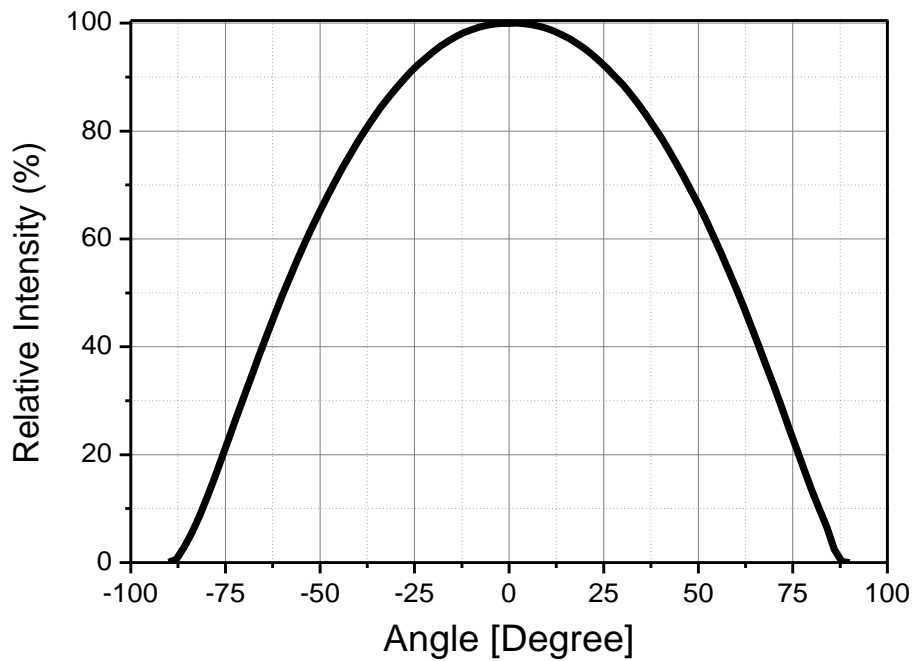
Fig 2. Viewing Angle Distribution, I_F=100\text{mA}
