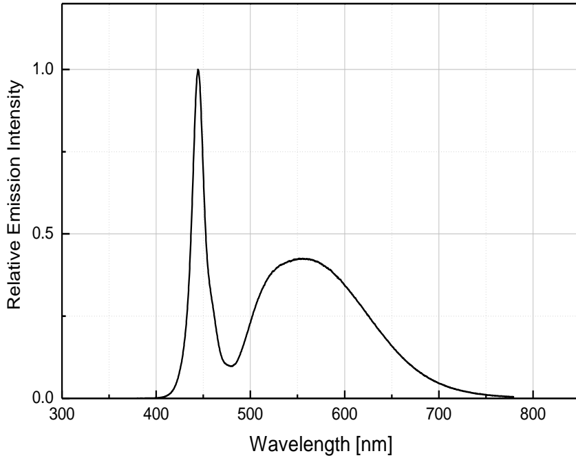
Fig 1. Color Spectrum, T_j = 25^\circ\text{C} , RH30%, I_F=100\text{mA}
